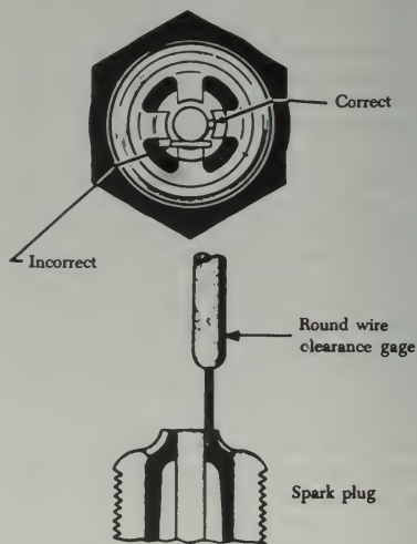
FIGURE 4-58. Use of a gap-measuring gage.
